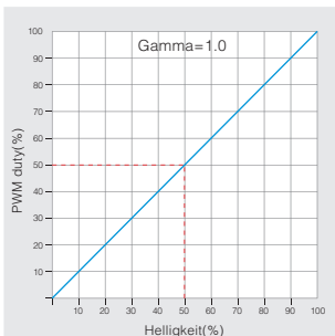
Lineare Dimmkurve
